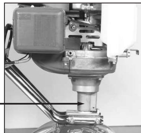
Picture 3... Note how the engine sits all the way down on the transmission.
